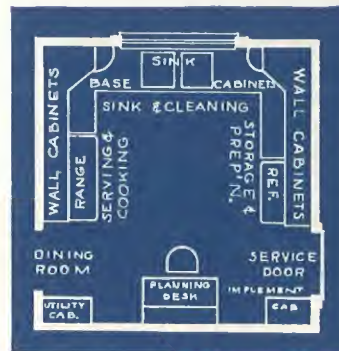
"U" SHAPE KITCHEN
